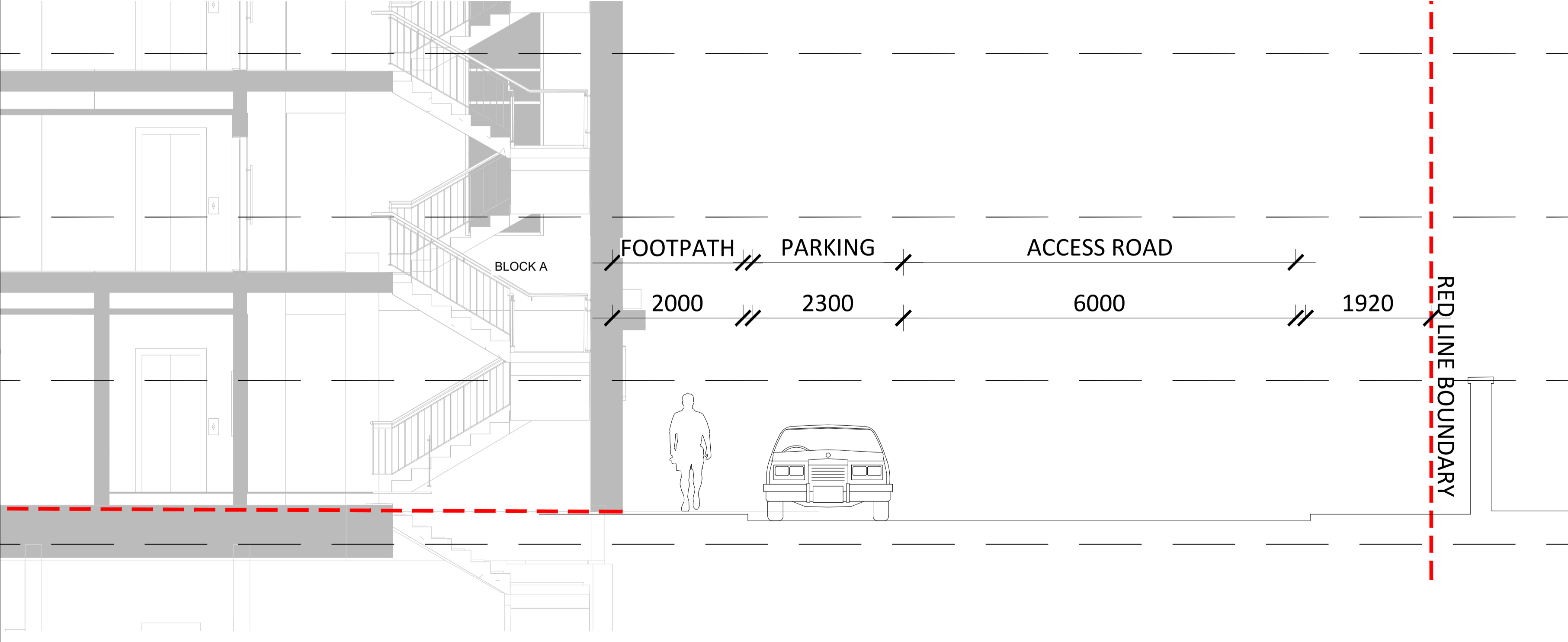
02 Landscape Section 04 Northern Boundary Section Scale 1:50
